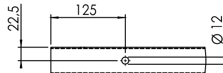
DETAIL B SCALE 1 : 5
